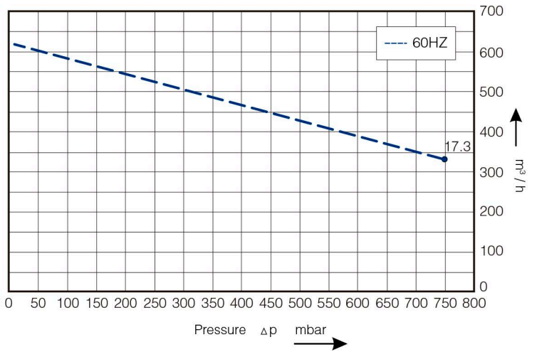
Pressure Selection Curve
